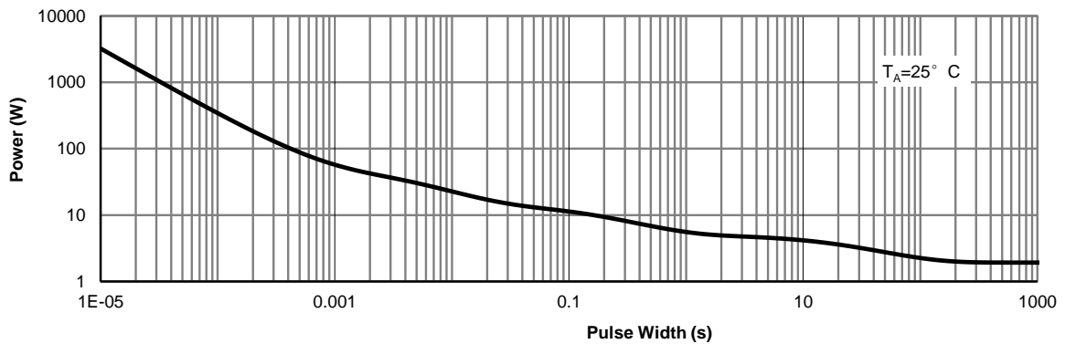
Figure 14: Single Pulse Power Rating Junction-to-Ambient (Note H)
