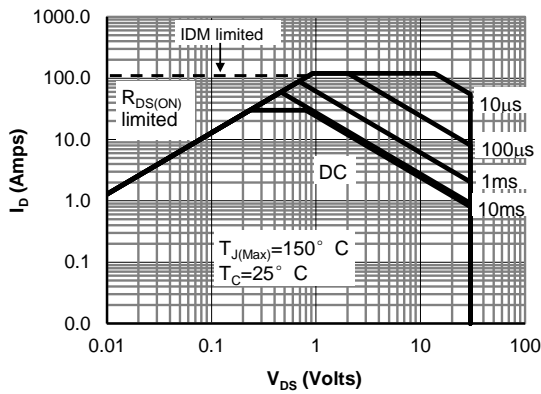
VGS > or equal to 4.5V Figure 9: Maximum Forward Biased Safe Operating Area (Note F)
