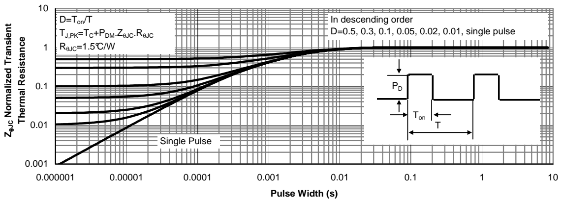
Figure 15: Normalized Maximum Transient Thermal Impedance for AOW4S60 (Note F)
