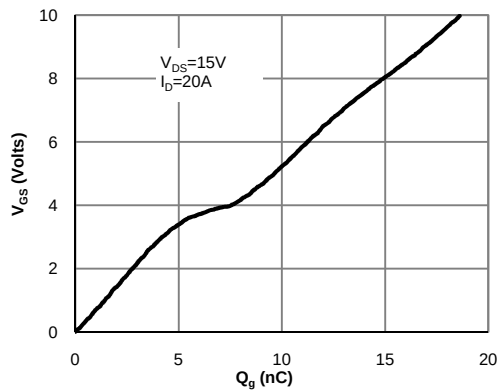
Figure 7: Gate-Charge Characteristics
