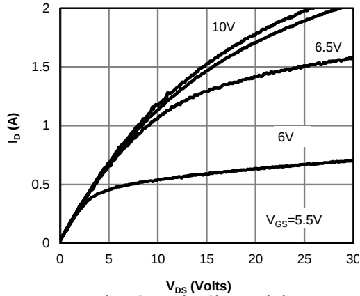
Fig 1: On-Region Characteristics
