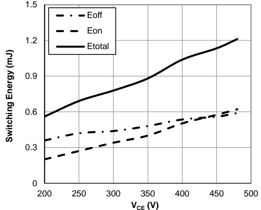
Figure 20: Switching Loss vs. V_{CE} ( T_j=150^\circ C, V_{GE}=15V, I_C=20A, R_{gon}=7.5\Omega, R_{goff}=47\Omega )
