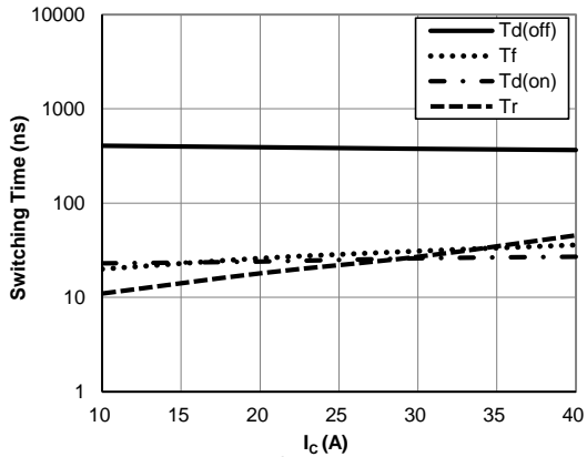
Figure 13: Switching Time vs. I_C ( T_J=150^{\circ}\text{C} , V_{GE}=15\text{V} , V_{CE}=400\text{V} , R_{gon}=7.5\Omega , R_{goff}=47\Omega )
