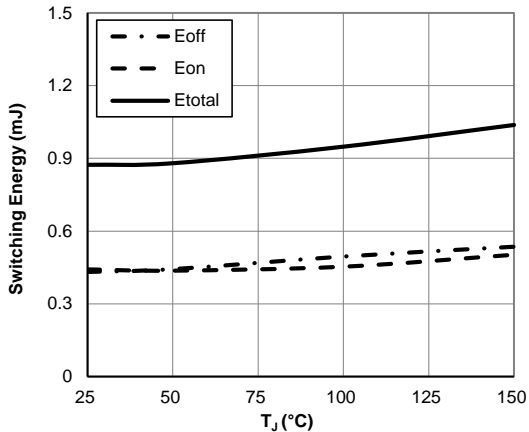
Figure 19: Switching Loss vs. T_j ( V_{GE}=15V, V_{CE}=400V, I_C=20A, R_{gon}=7.5\Omega, R_{goff}=47\Omega )
