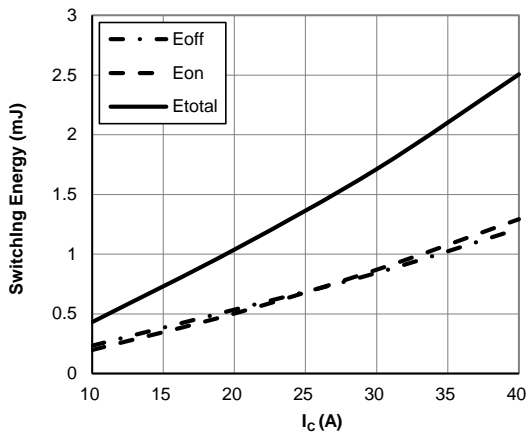
Figure 17: Switching Loss vs. I_C ( T_J=150^{\circ}\text{C} , V_{GE}=15\text{V} , V_{CE}=400\text{V} , R_{gon}=7.5\Omega , R_{goff}=47\Omega )
