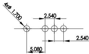
RECOMMENDED THROUGH HOLES FOR LAND PATTERN
