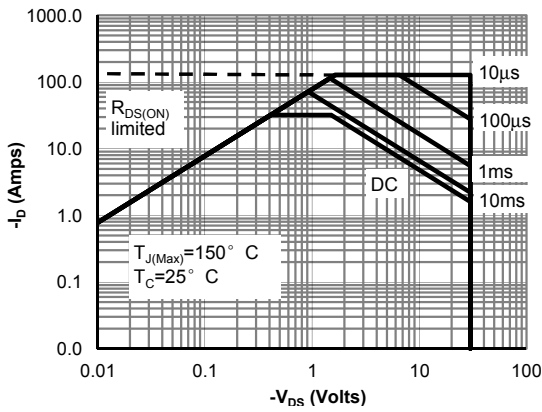
Figure 9: Maximum Forward Biased Safe Operating Area (Note F) V_{GS} > \text{or equal to } 4.5V
