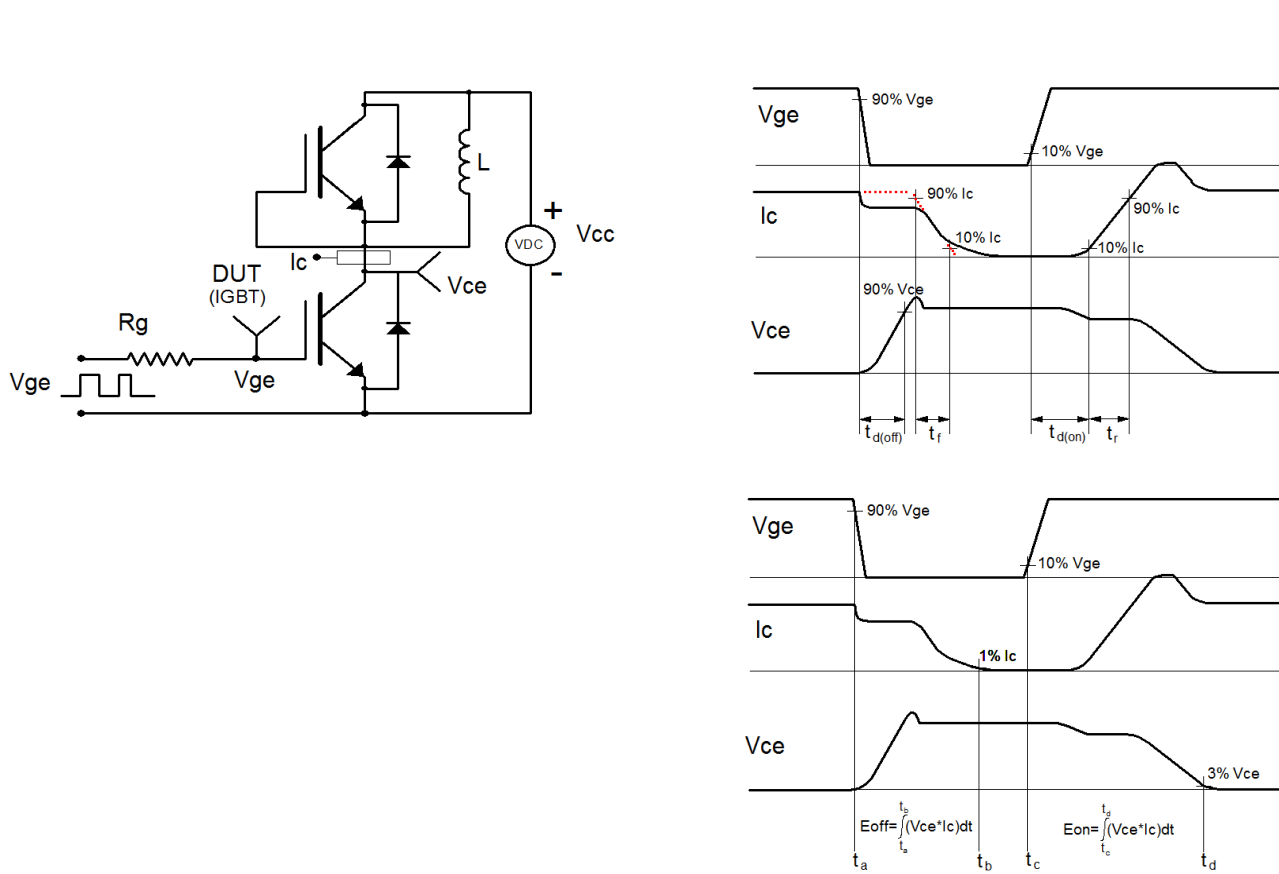
Figure B: Inductive Switching Test Circuit & Waveforms
