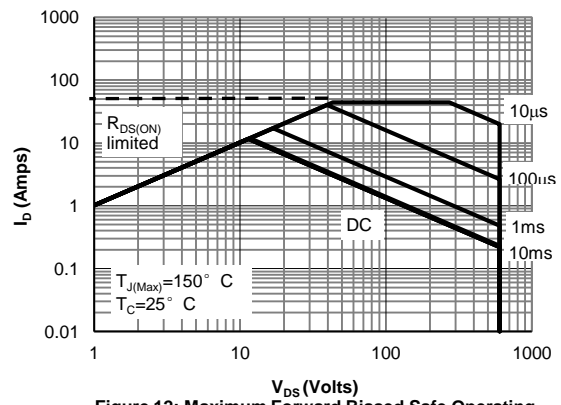
Figure 12: Maximum Forward Biased Safe Operating Area for AOT380A60L (Note F)
