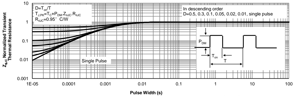
Figure 14: Normalized Maximum Transient Thermal Impedance for AOT380A60L (Note F)
