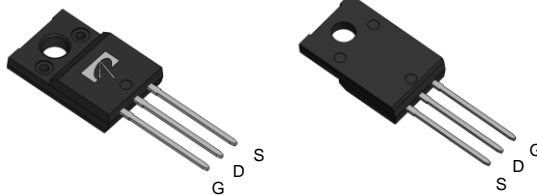
TO-220FNL
