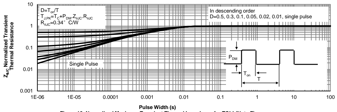
Figure 12: Normalized Maximum Transient Thermal Impedance for TOLL(Note F)
