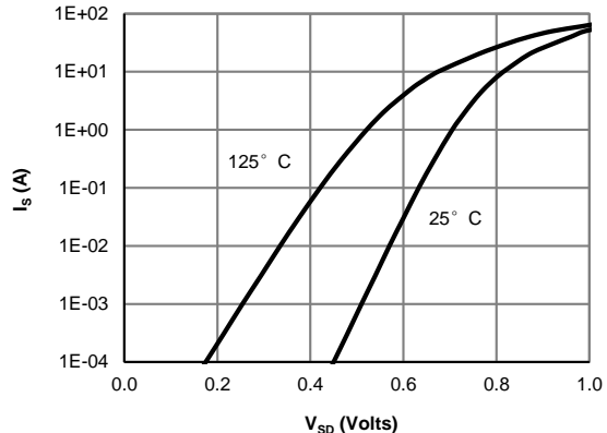
Figure 6: Body-Diode Characteristics
