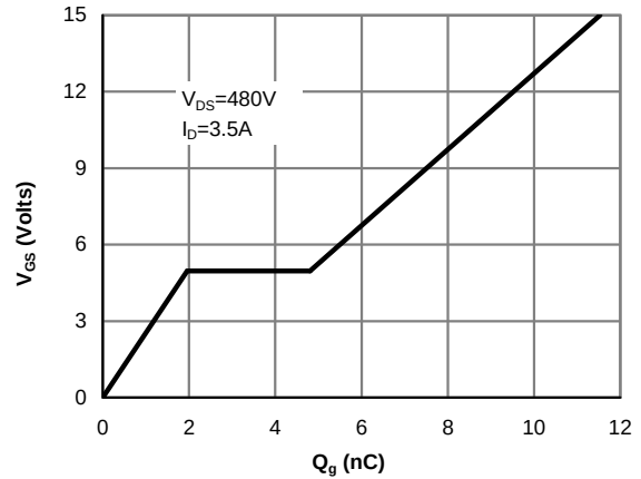
Figure 8: Gate-Charge Characteristics
