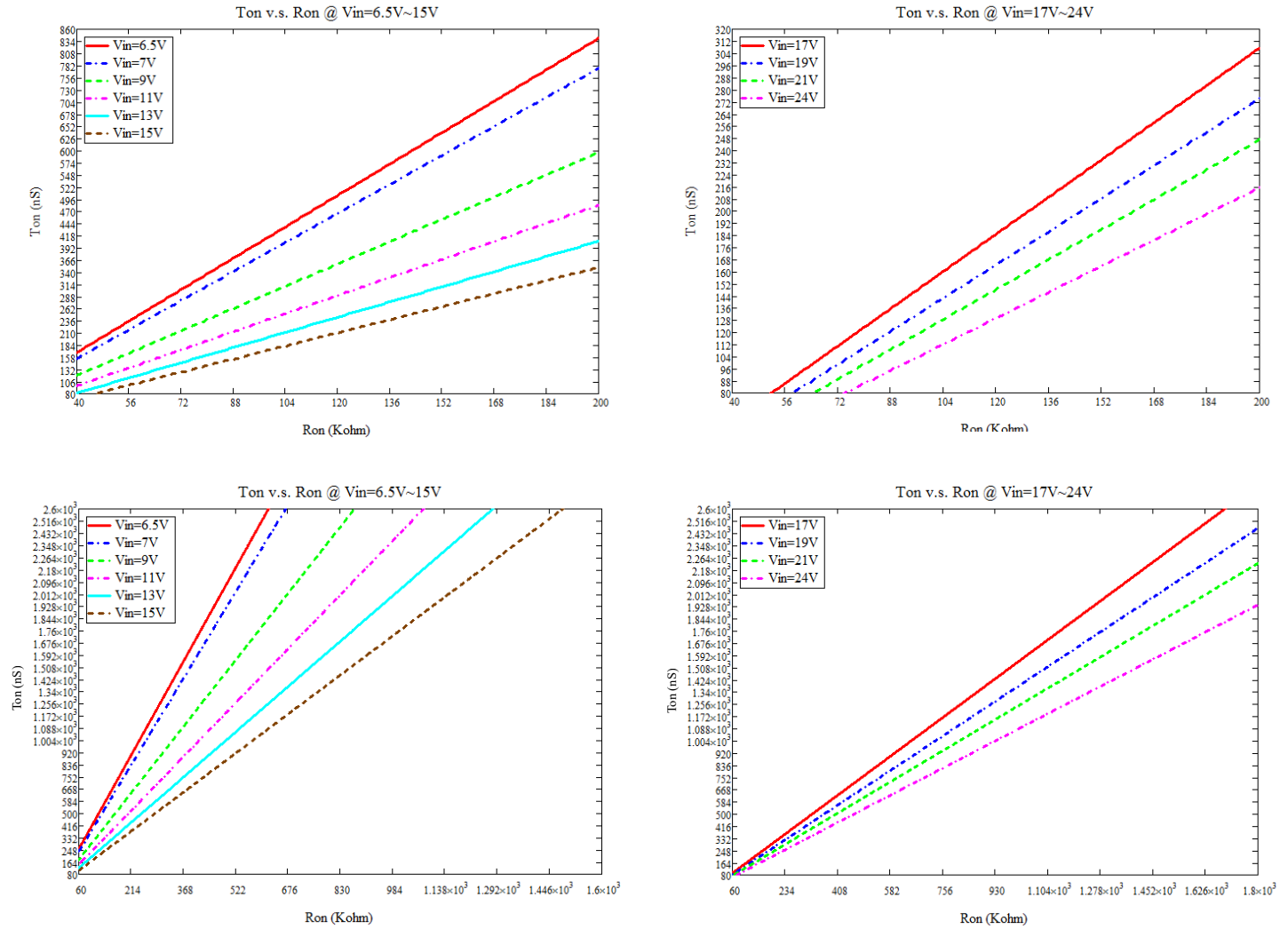
Figure 3. T_{on} vs. R_{on} Curves for AOZ22555QI
