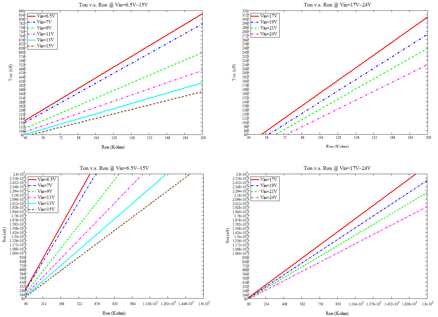
Figure 3. T_{on} vs. R_{ton} Curves for AOZ22557QI
