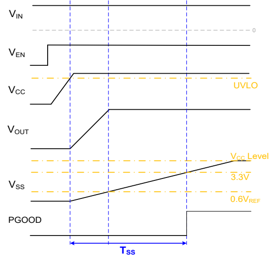
Figure 1. Soft Start Sequence of AOZ22557QI
