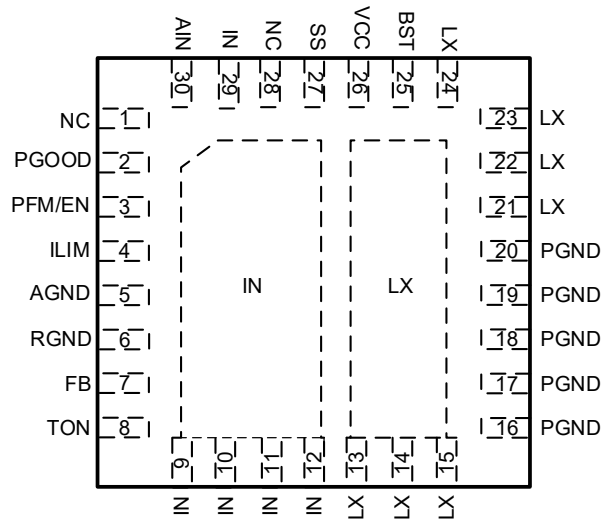
AOZ22557QI 30-Pin 4mm x 4mm QFN
