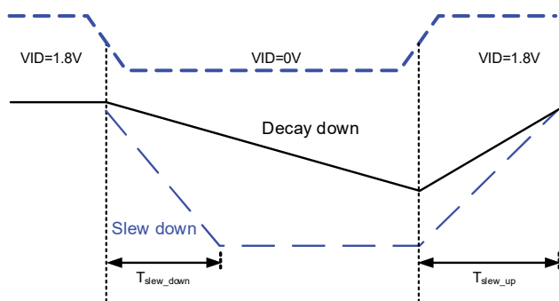
Figure 5. Decay Mode Illustration
