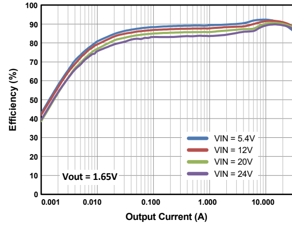
Figure 2. Efficiency vs. Load Current ( V_{OUT}=1.65V )
