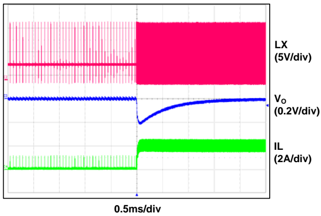
PEM to PWM Transition
