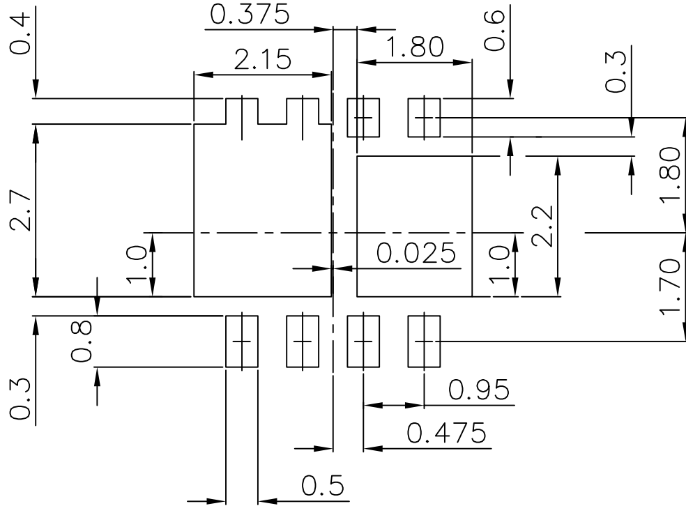
RECOMMENDED LAND PATTERN (UNIT: mm)
