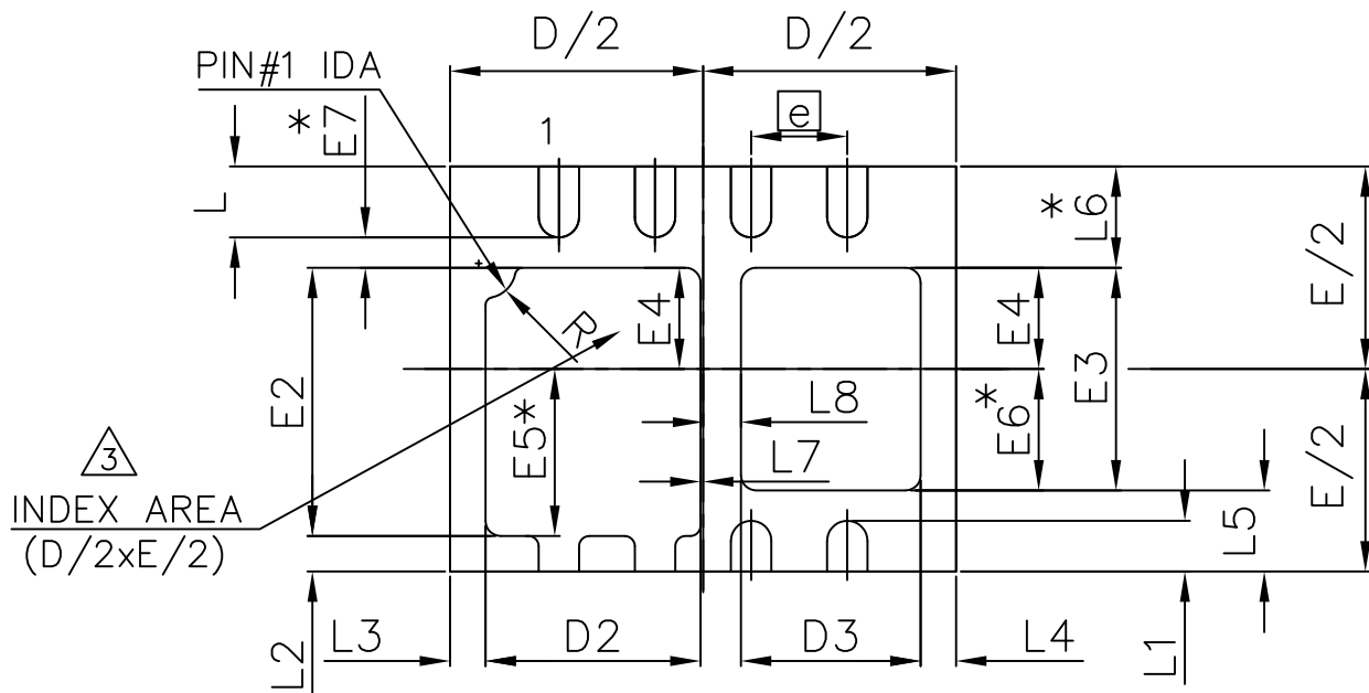
BOTTOM VIEW
