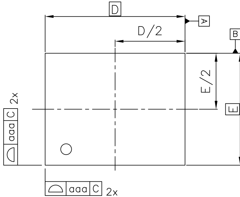
6 TOP VIEW
