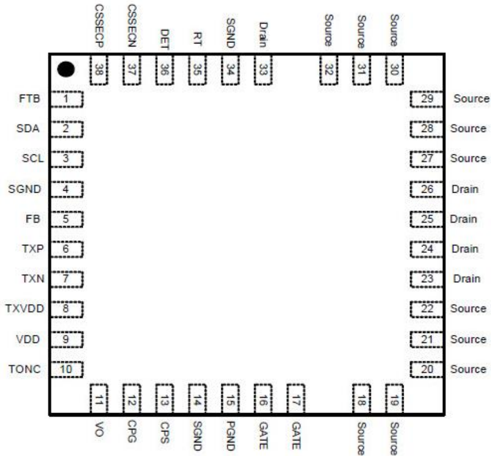
38-Pin 6mmx6mm QFN (Top View)
