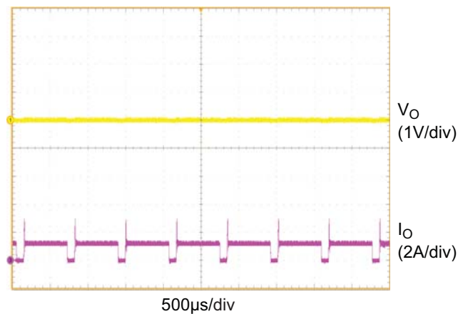
Short Current Protection
