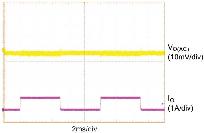
Load Transient Response (1A)
