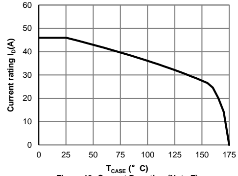
Figure 13: Current De-rating (Note F)
