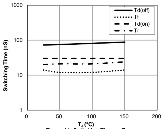
Figure 14: Switching Time vs. T_J ( V_{GE}=15\text{V}, V_{CE}=400\text{V}, I_C=40\text{A}, R_g=7.5\Omega )
