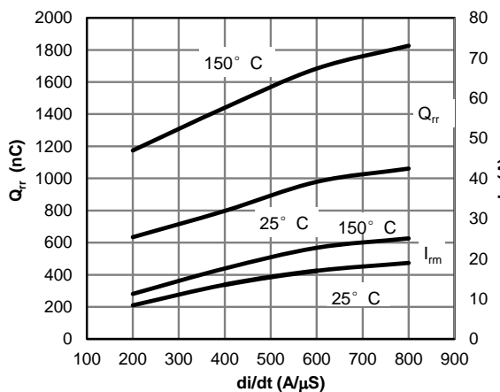
Fig 23: Diode Reverse Recovery Charge and Peak Current vs. di/dt ( V_{GE}=15V, V_{CE}=400V, I_F=20A )
