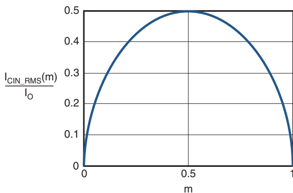
Figure 5. I_{CIN} vs. Voltage Conversion Ratio
