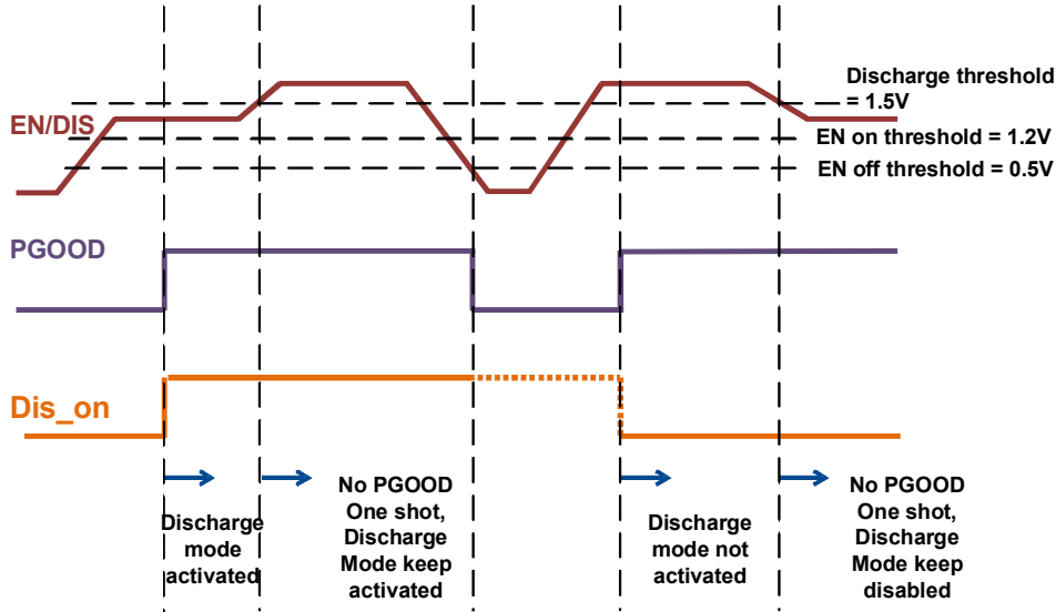
Figure 2. AOZ2262NQL-11 Discharge Function On/Off Setting
