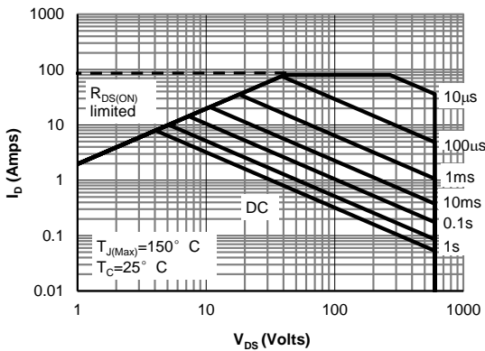
Figure 11: Maximum Forward Biased Safe Operating Area for AOTF190A60CL (Note F)
