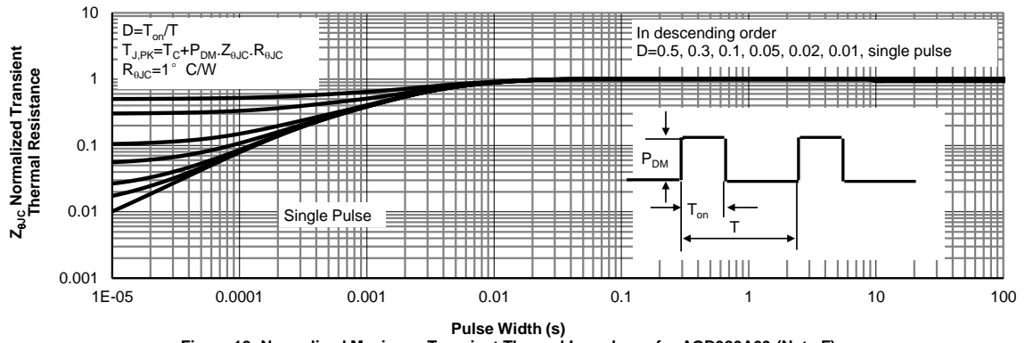
Figure 12: Normalized Maximum Transient Thermal Impedance for AOD380A60 (Note F)
