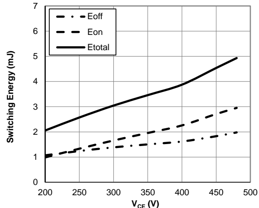
Figure 20: Switching Loss vs. V_{CE} ( T_j=175^\circ C , V_{GE}=15V , I_C=60A , R_g=5\Omega )
