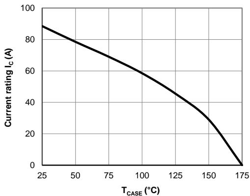
Figure 11: Current De-rating
