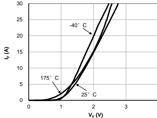
Figure 4: Diode Characteristic
