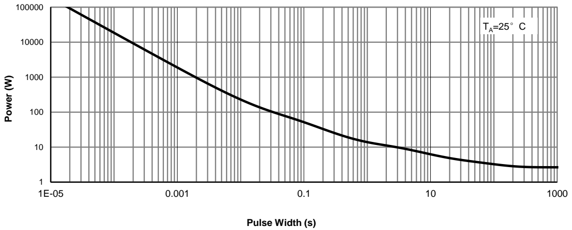
Figure 13: Single Pulse Power Rating Junction-to-Ambient (Note G)
