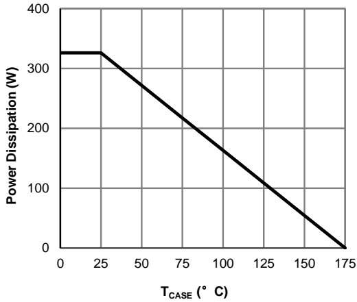
Figure 11: Power De-rating (Note F)
