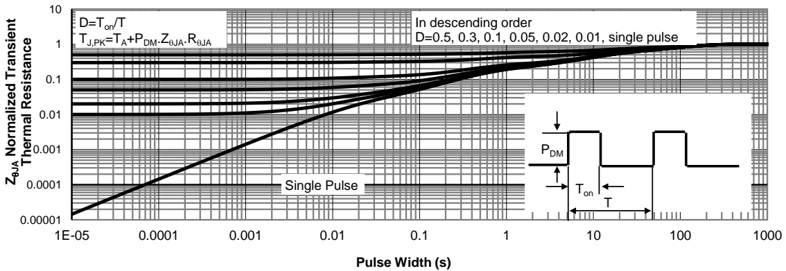
Figure 14: Normalized Maximum Transient Thermal Impedance (Note G)
