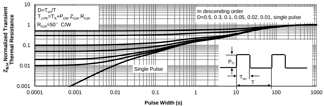
Figure 15: Normalized Maximum Transient Thermal Impedance (Note G)
