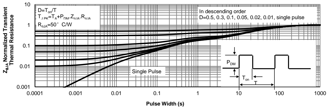
Figure 16: Normalized Maximum Transient Thermal Impedance (Note G)
