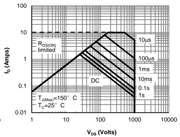
Figure 10: Maximum Forward Biased Safe Operating Area for AOTF3N100 (Note F)
