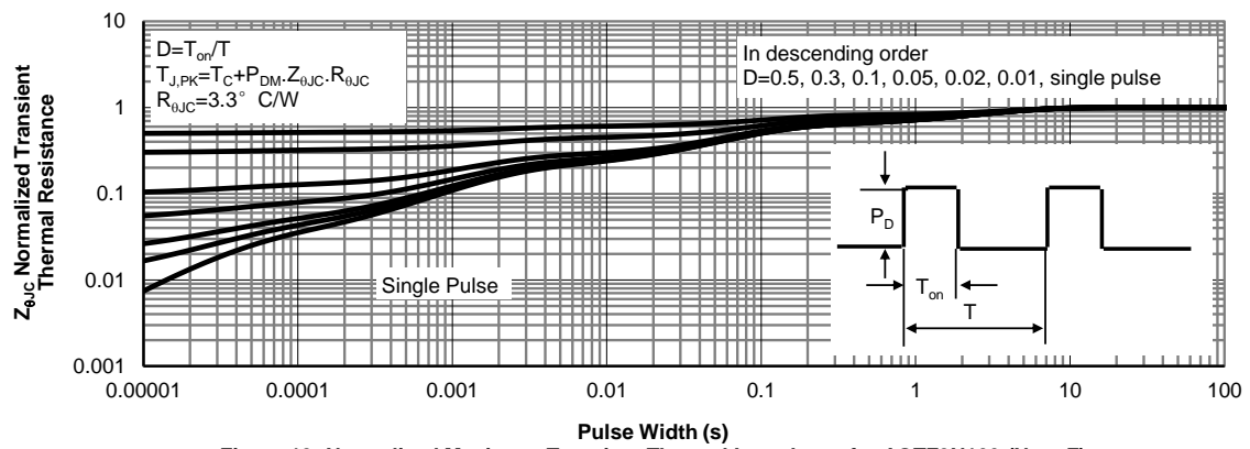
Figure 13: Normalized Maximum Transient Thermal Impedance for AOTF3N100 (Note F)
