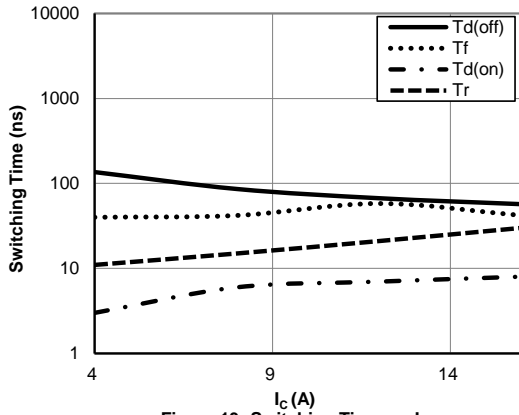
Figure 13: Switching Time vs. I_C ( T_J=175^\circ\text{C} , V_{GE}=15\text{V} , V_{CE}=400\text{V} , R_g=37.5\Omega )
