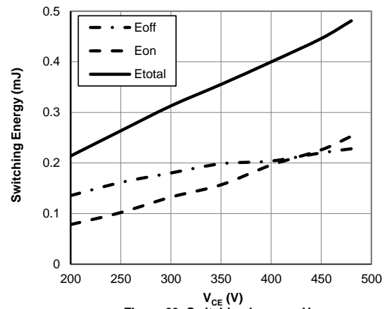
Figure 20: Switching Loss vs. V_{CE} ( T_j=150^\circ\text{C} , V_{GE}=15\text{V} , I_c=10\text{A} , R_g=30\Omega )
