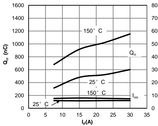
Figure 22: Diode Reverse Recovery Charge and Peak Current vs. Conduction Current ( V_{GE}=15V, V_{CE}=400V, di/dt=200A/\mu s )
