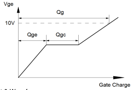
Figure A: Gate Charge Test Circuit & Waveforms
