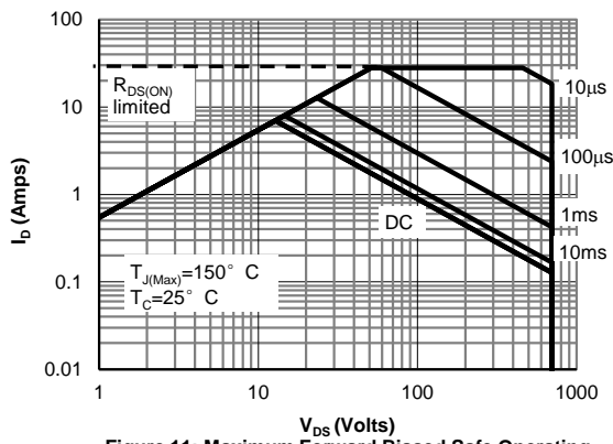
Figure 11: Maximum Forward Biased Safe Operating Area for AOT(B)780A70L (Note F)
