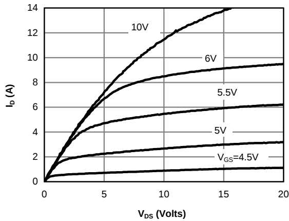
Figure 1: On-Region Characteristics@25°C
