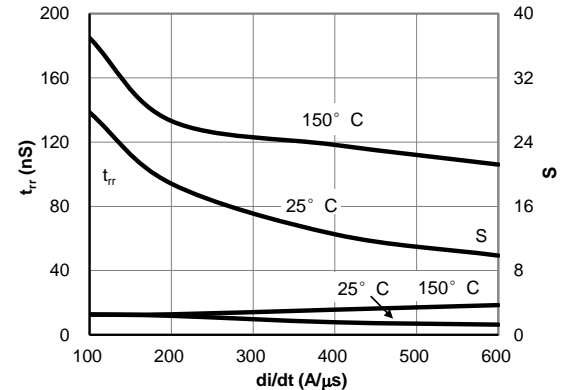
Figure 24: Diode Reverse Recovery Time and Softness Factor vs. di/dt ( V_{GE}=15V, V_{CE}=400V, I_F=8A )
