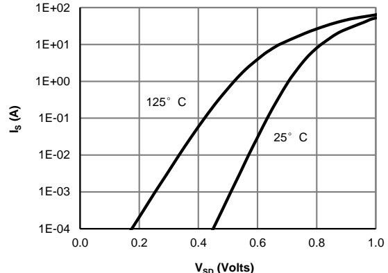
Figure 6: Body-Diode Characteristics
