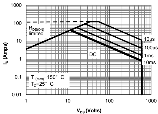
Figure 11: Maximum Forward Biased Safe Operating Area for TOLL (Note F)
