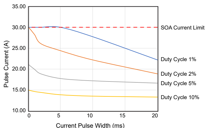
Figure 17. AOZ13287DI-03 Sinking Switch Pulsed Current vs. Duration for a Given Duty Cycle
