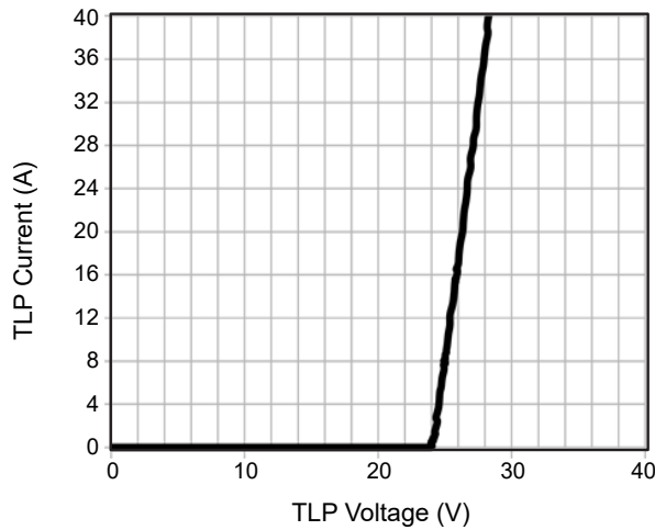
Figure 10. Positive Curve IEC61000-4-5 Surge 8/20 \mu s
