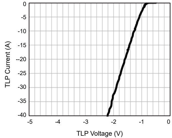
Figure 11. Negative Curve IEC61000-4-5 Surge 8/20 \mu s
