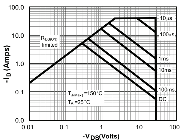
Internal Power MOSFET SOA
