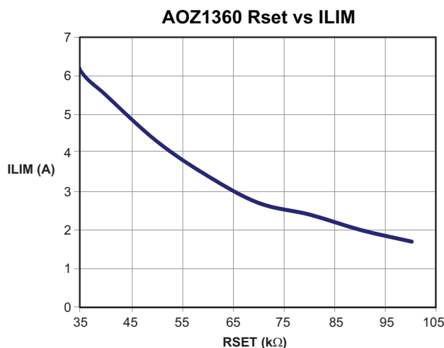
Figure 3. Current Limit vs. RSET
