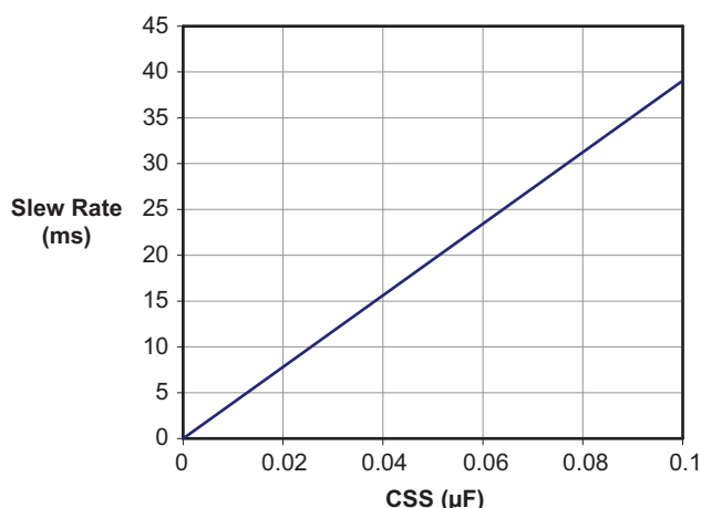
Figure 4. Output Slew Rate vs. CSS
