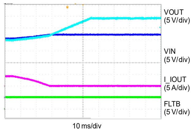
Ideal Diode True Reverse Current Blocking ( V_{IN} = 20\text{V} , R_{OUT} = 4\Omega )
