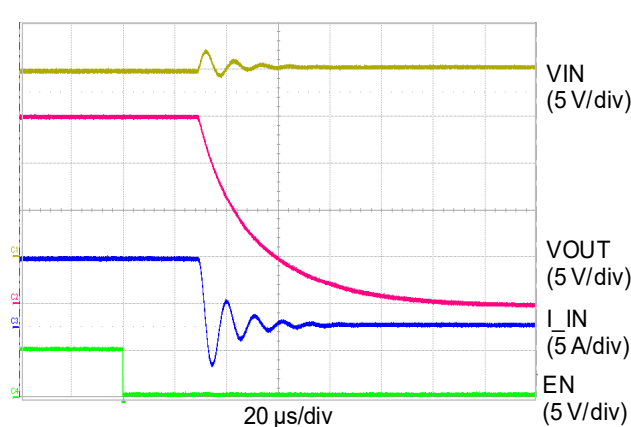
Shut Down ( V_{IN} = 20\text{V} , R_{OUT} = 2.8\Omega )
