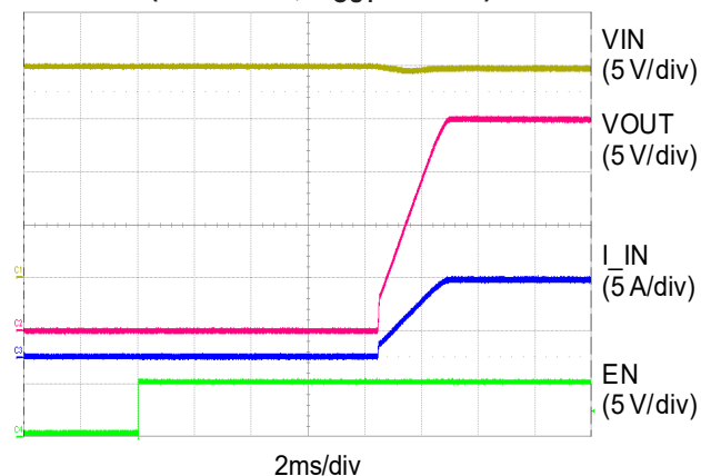
Soft Start Delay Time ( V_{IN} = 20\text{V} , R_{OUT} = 2.8\Omega )
