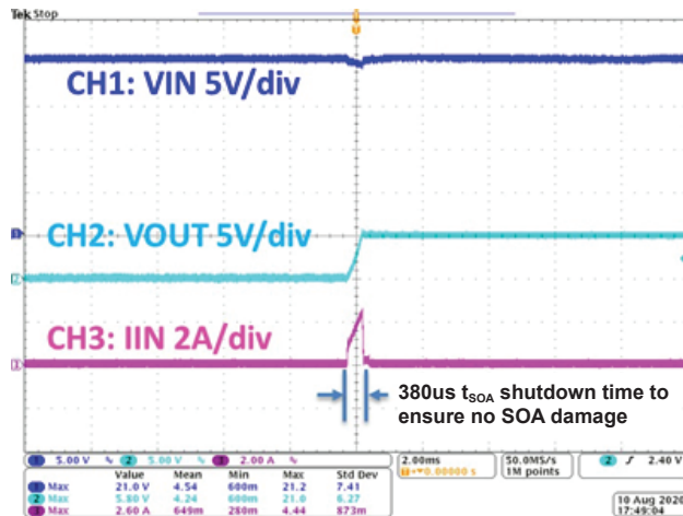
Figure 13(a). AOZ13987DI-03/04 Shuts Down after Current Clamps for 380 \mu s, C_{SS} =5.6 nF, C_{OUT} = 150 \mu F, No Load
