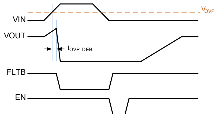
Figure 2. Over-Voltage Protection
