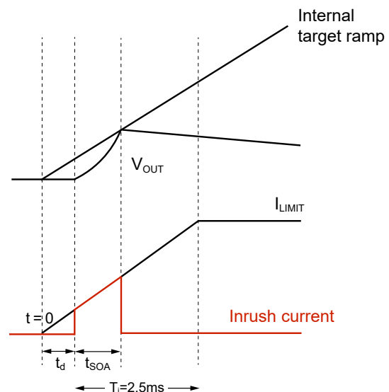
Figure 12. AOZ13987DI-03/04 Startup Current Limit and SOA Shutdown Scheme
