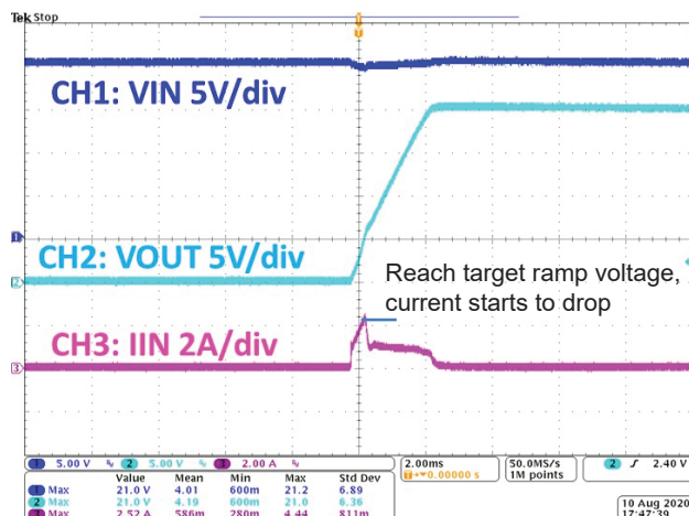
Figure 13(b). AOZ13987DI-03/04 Normal Startup without Shutdown C_{SS} =5.6 nF, C_{OUT} = 140 \mu F, No Load
