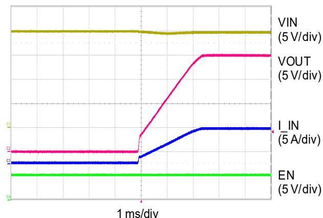
Soft Start Ramp ( V_{IN} = 20\text{V} , R_{OUT} = 2.8\Omega )
