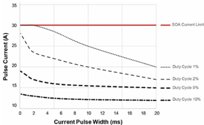
Figure 11. AOZ13987DI-03/04 Sinking Switch Pulsed Current vs. Duration for a Given Duty Cycle
