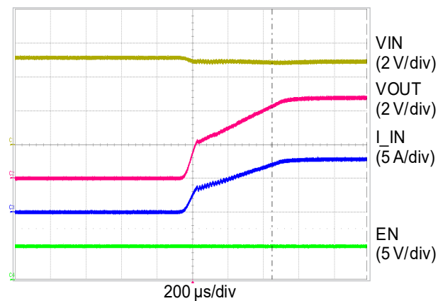
Soft Start Ramp ( V_{IN} = 5\text{V} , R_{OUT} = 0.6\Omega )
