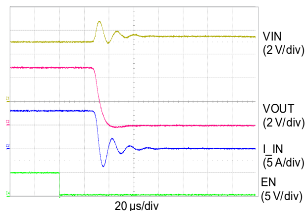
Shut Down ( V_{IN} = 5\text{V} , R_{OUT} = 0.6\Omega )
