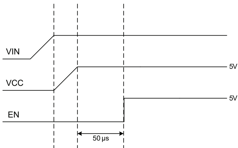
Figure 1. Start-up Sequence
