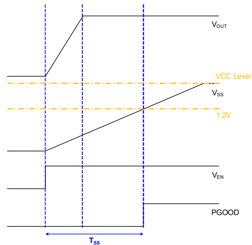
Figure 1. Soft-Start Sequence of AOZ2263NQi-11
