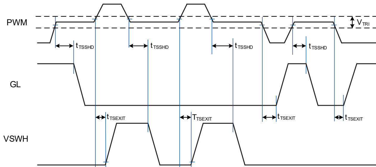
Figure 2. Over-Voltage Protection
