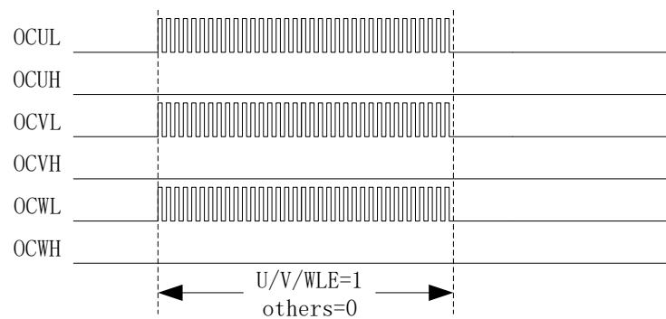
Figure 19-7 Brake Waveform
