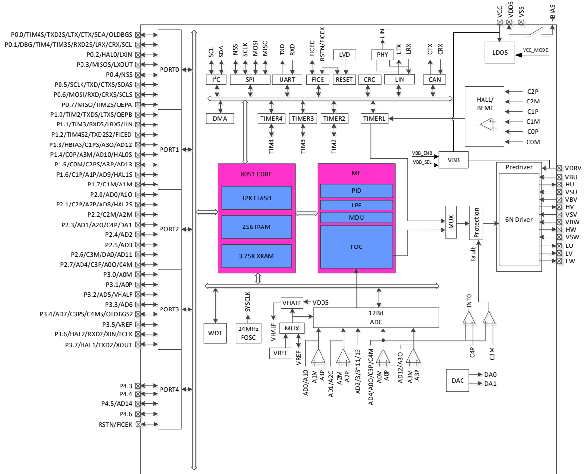
Figure 1-1 Functional Block Diagram of AOZ6866QI
