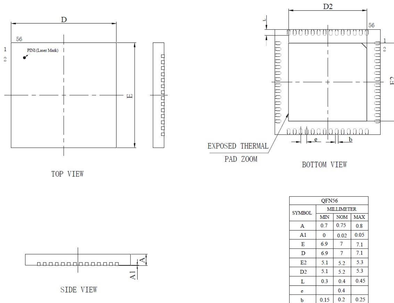
Figure 3-1 AOZ6866QI QFN56_7X7 Package Drawings and Dimensions
