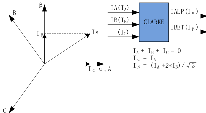
Figure 14-3 Clarke Transformation
