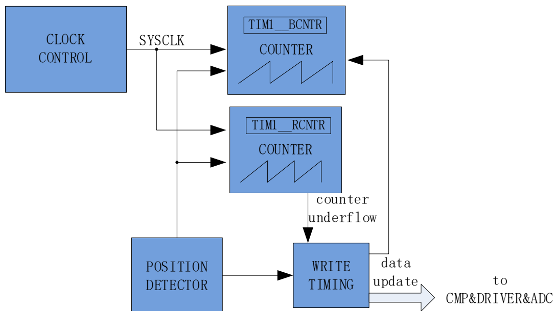
Figure 15-1 Timer1 Internal Structure
