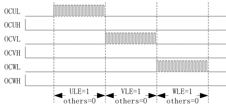
Figure 19-6 Pre-charge Waveform
