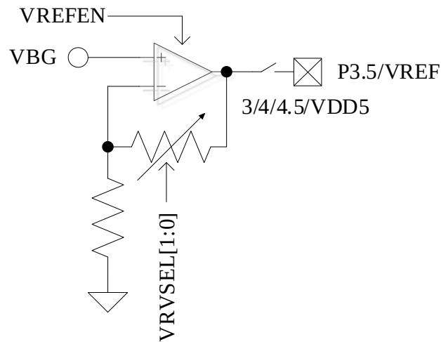
Figure 28-1 I/O Pins of VREF Module
