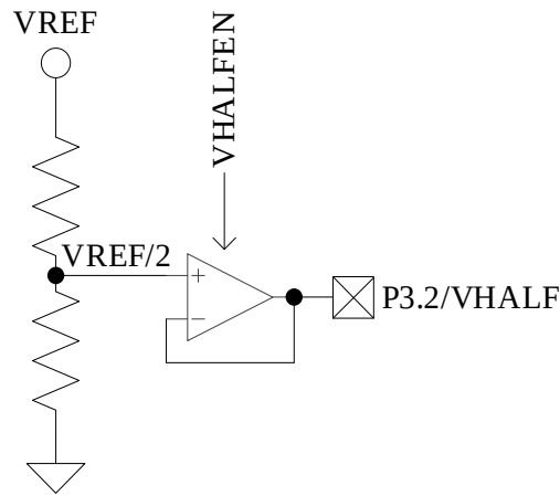
Figure 29-1 I/O Pins of VHALF Module
