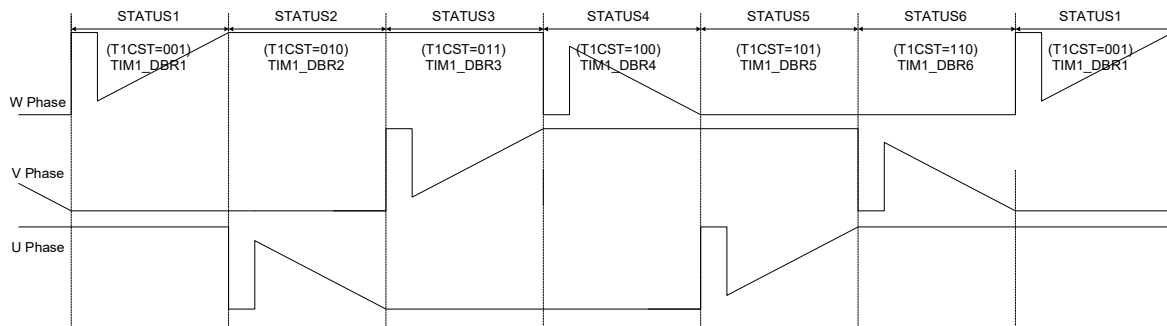
Figure 15-11 Diagram of Six-step Phase Commutation of Square Wave Control
