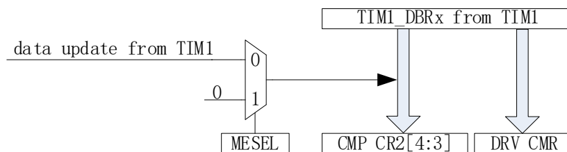
Figure 19-5 Timer1 Automatic Control of DRV_CM and CMP_CR2[4:3]
