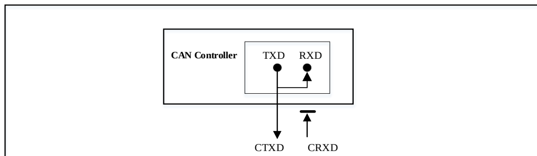
Figure 12-11 Self-test Mode
