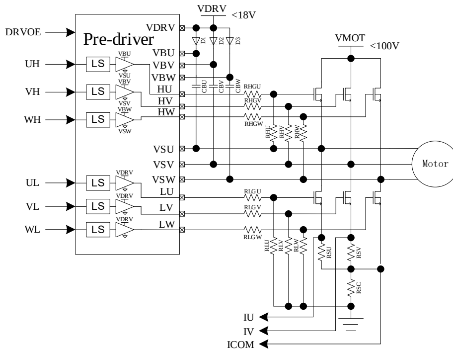
Figure 19-9 Block Diagram of 6N Pre-driver Mode
