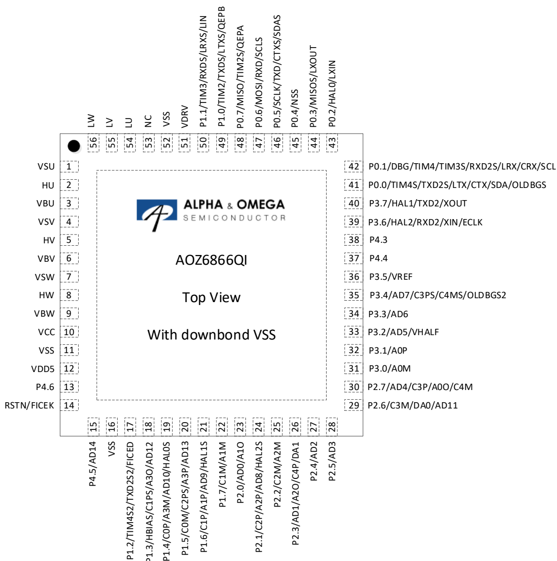
Figure 2-1 AOZ6866QI QFN56 Pinout Diagram
