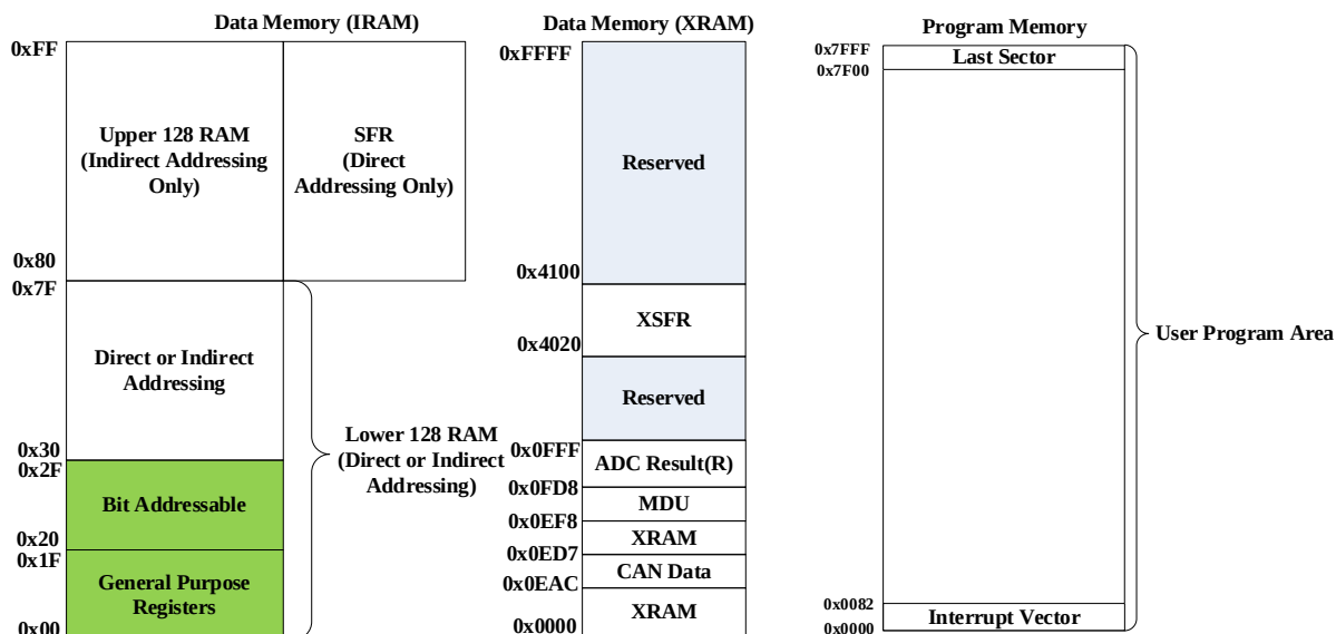
Figure 1-2 Memory Organization
