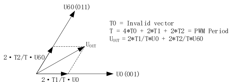
Figure 14-6 SVPWM Voltage Vector Synthesis
