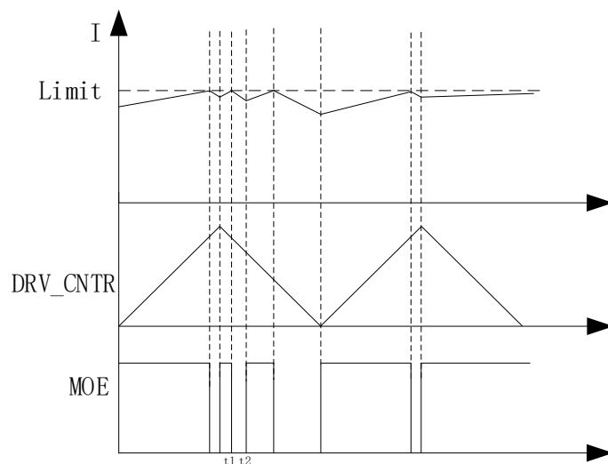
Figure 31-6 Cycle-by-cycle Current Limiting Waveform ( t_2 - t_1 = 5\mu s ) when EVT_FILT[MOEMD] = 11
