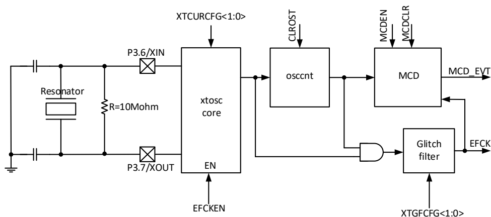
Figure 23-2 Crystal Input Mode of External Fast Clock
