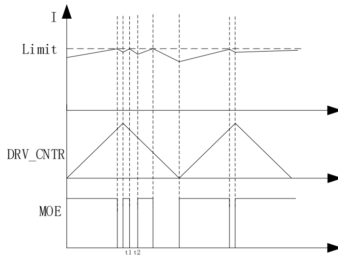
Figure 31-5 Cycle-by-cycle Current Limiting Waveform ( t_2 - t_1 = 10\mu s ) when EVT_FILT[MOEMD] = 10
