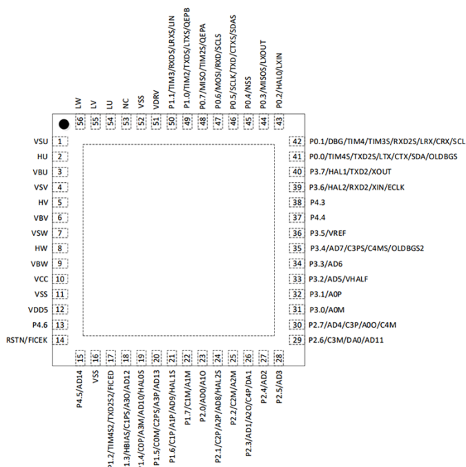
QFN7x7-56L
