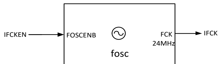
Figure 23-1 Input/Output of Internal Fast Clock
