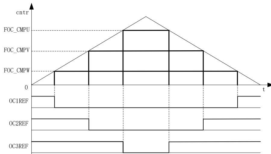
Figure 19-3 PMW Generation
