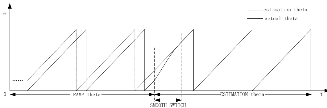
Figure 14-15 Angle Smooth Switching Curve
