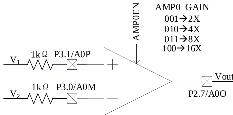
Figure 30-3 AMP0 Operating in PGA Differential Input Mode
