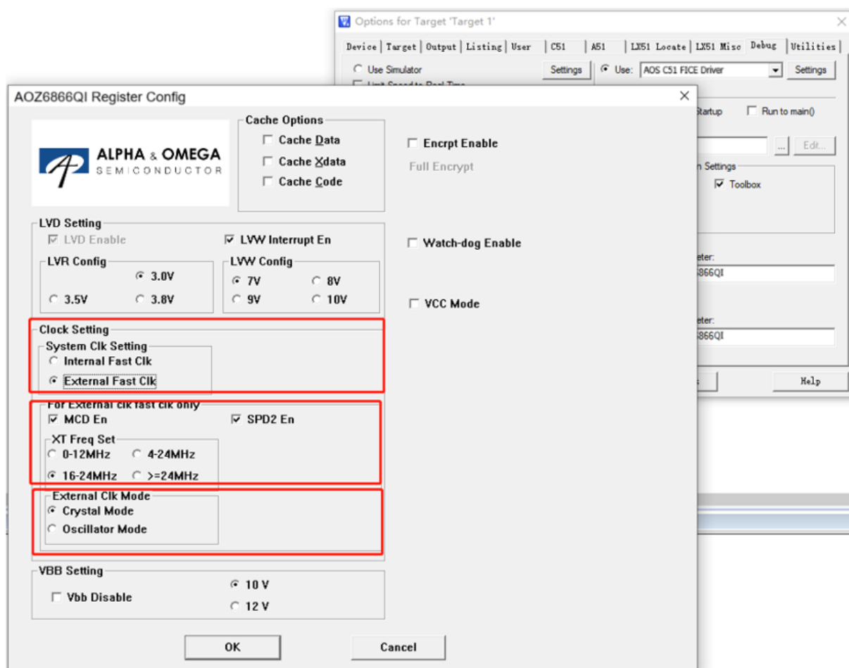
Figure 23-6 AOZ6866QI SYSCLOCK Configure
