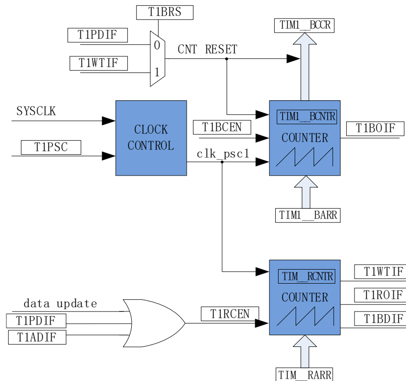
Figure 15-2 Timebase Unit
