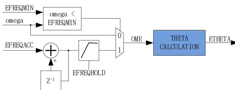
Figure 14-14 Schematic Diagram of Forced Angle of Estimator
