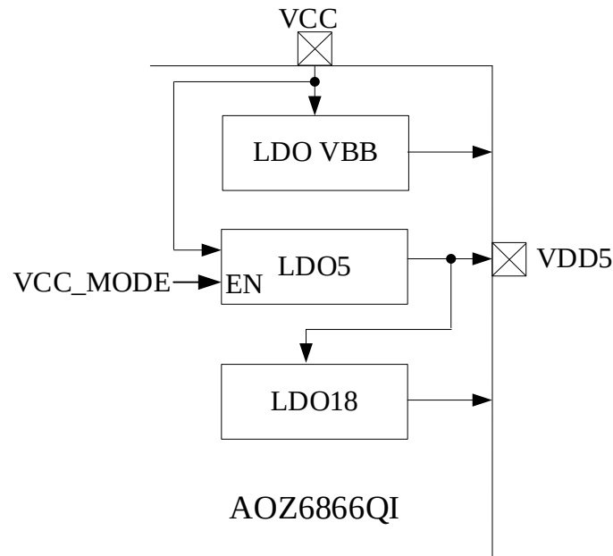
Figure 32-1 Functional Block Diagram of Power Supply for AOZ6866QI
