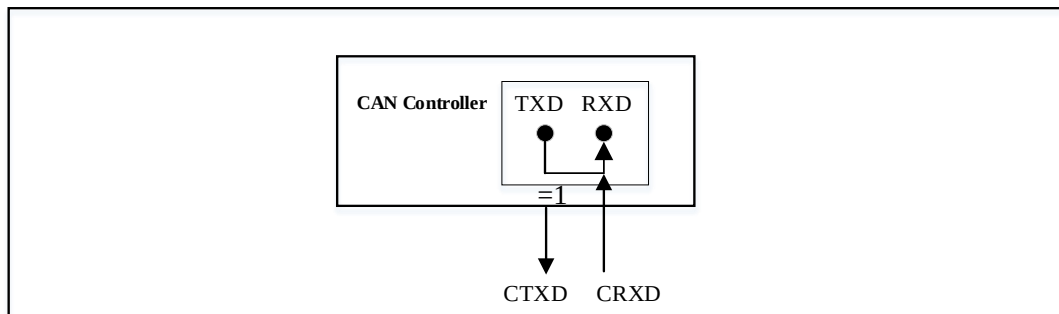
Figure 12-12 Monitoring Mode
