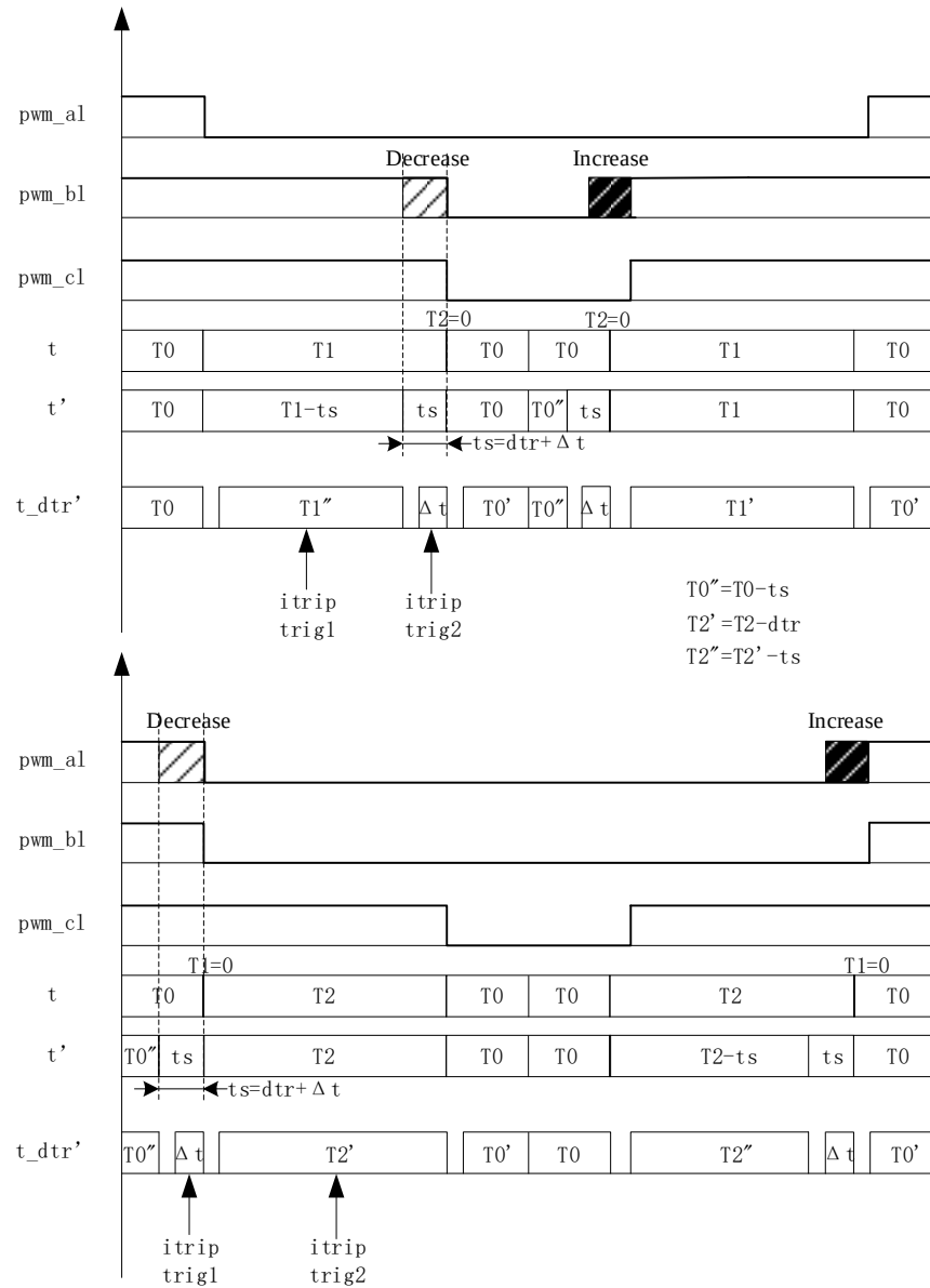
Figure 14-10 Time Compensation for Single-shunt Current Sampling
