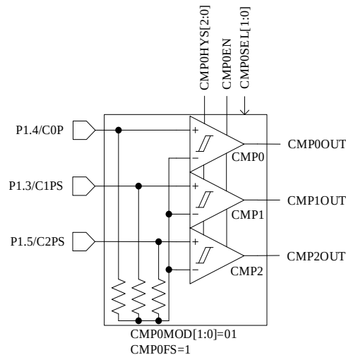
Figure 31-10 CMPG with Built-in Three Comparators and Resistors (with Function Switching)
