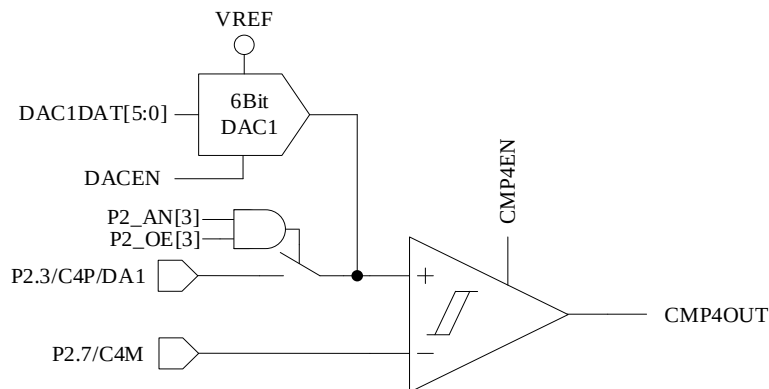
Figure 31-7 Schematic Diagram of CMP4 Module
