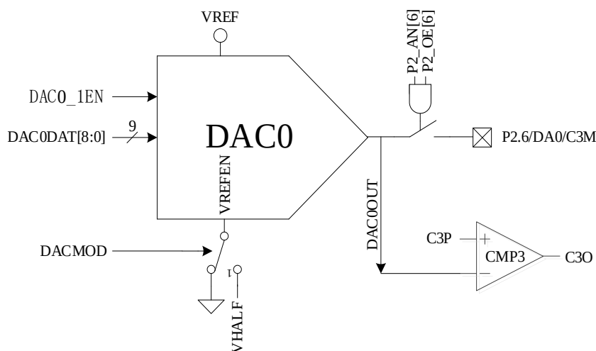
Figure 26-1 DAC0 Functional Block Diagram
