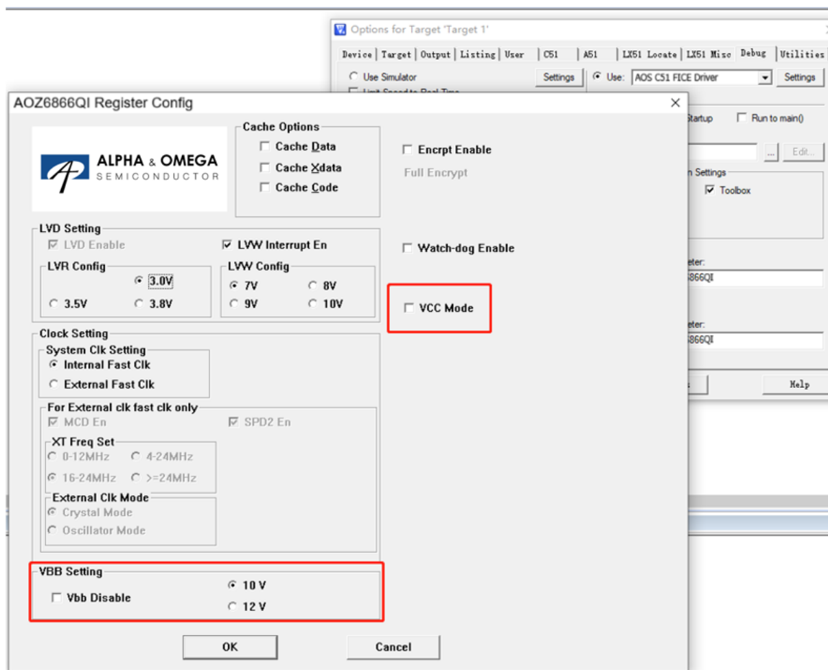
Figure 32-2 VCC_MODE Configurations for AOZ6866QI
