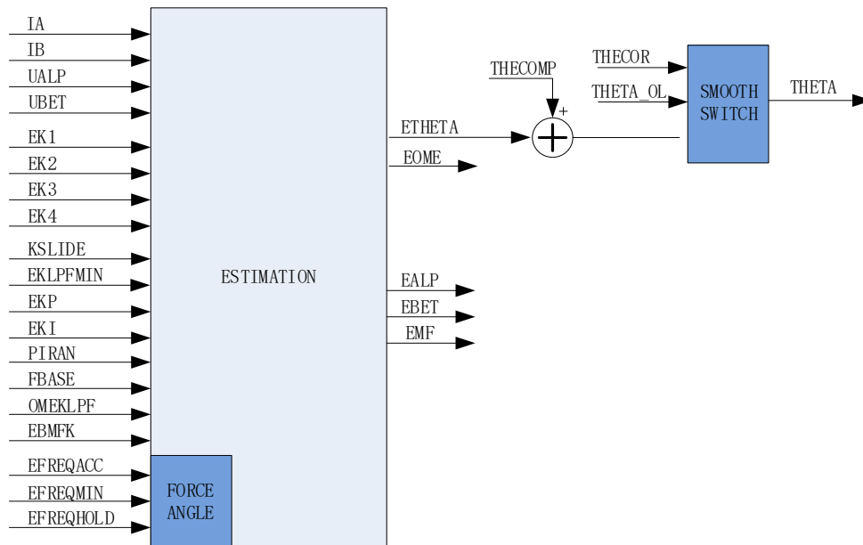
Figure 14-13 Schematic Block Diagram of Estimator
