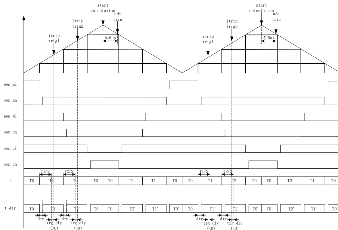
Figure 14-9 Single-shunt Current Sampling Timing
