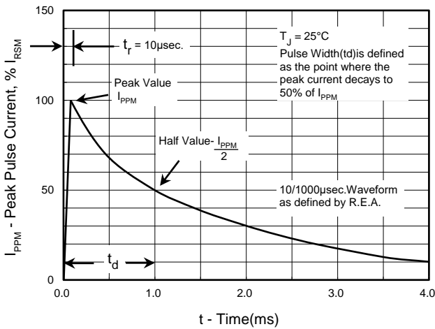
Pulse Waveform
