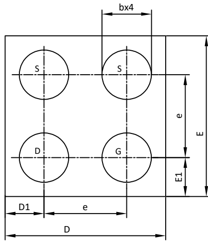
BUMP UP
