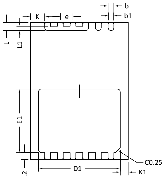
BOTTOM VIEW
