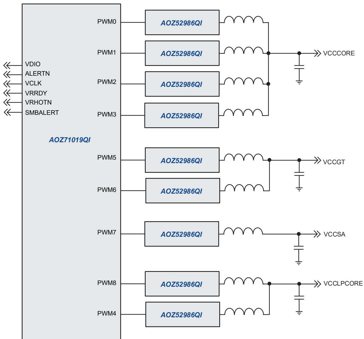
Figure 1. Typical Application
