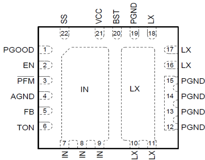
22-Pin 4 mm x 4 mm QFN (Top View)
