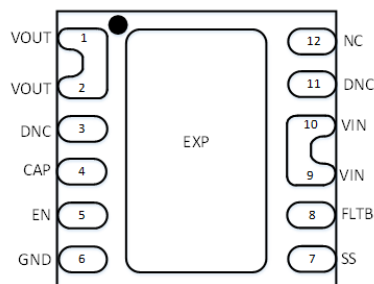
3mm x 3mm DFN-12L (Top Transparent View)
